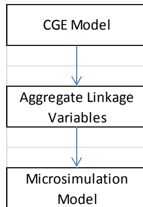
Figure 2.2: the Macro-Micro approach
