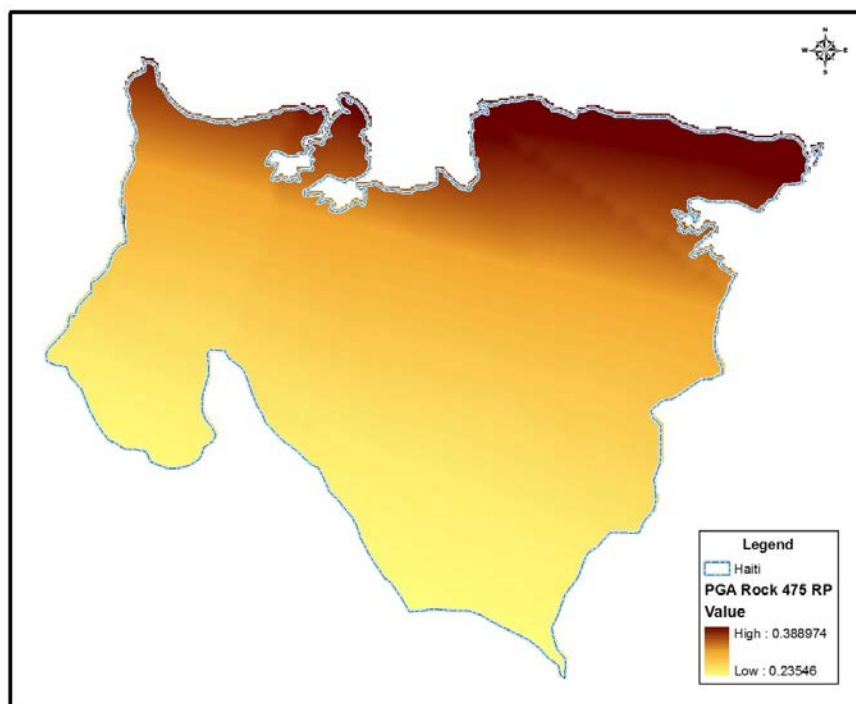
Figure A4.5 Distribution of PGA (in g) with 10% probability of exceedance in 50 years (475 years return periods) for the study area
