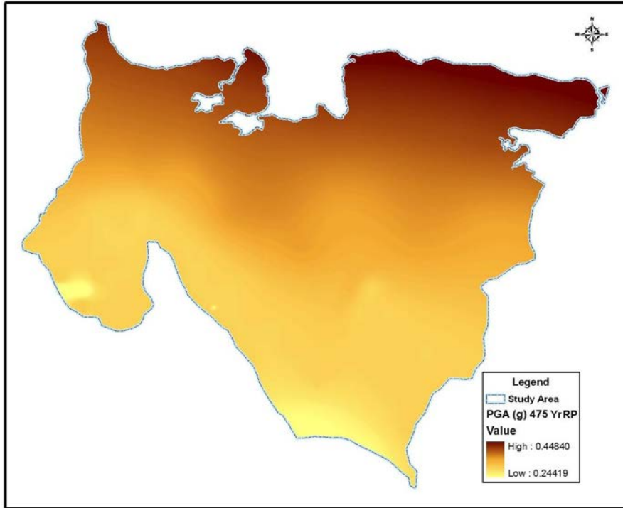
Figure A4.11 PGA probabilistic seismic hazard map for 10% probability in 50 years, i.e. 475-year return period
