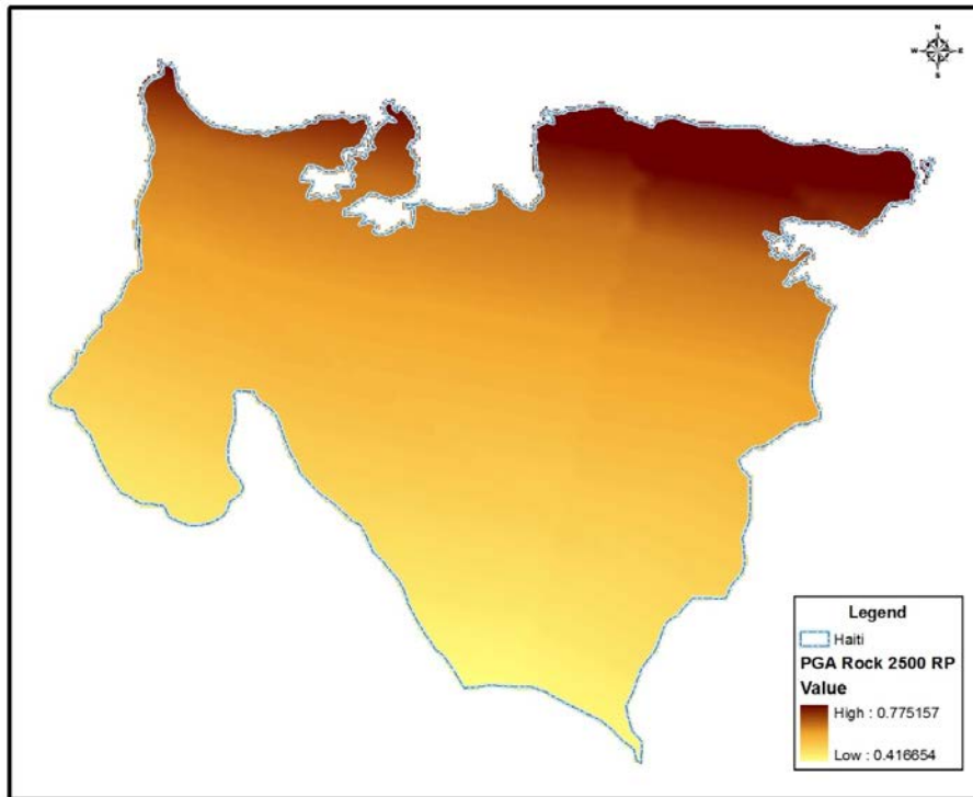
Figure A4.6 Distribution of PGA (in g) with 2% probability of exceedance in 50 years (2500 years return periods)
