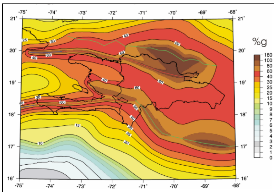
Figure A4.4 PGA (%g) with 2% probability of exceedance in 50 years (2500 years return periods)
