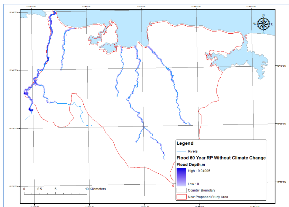
Figure A4.23 Flood Hazard Map without Climate Change 50 year return period
