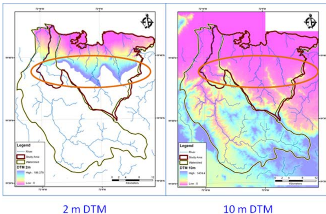
Figure A4.17 Two different DTMs available for study area and beyond
