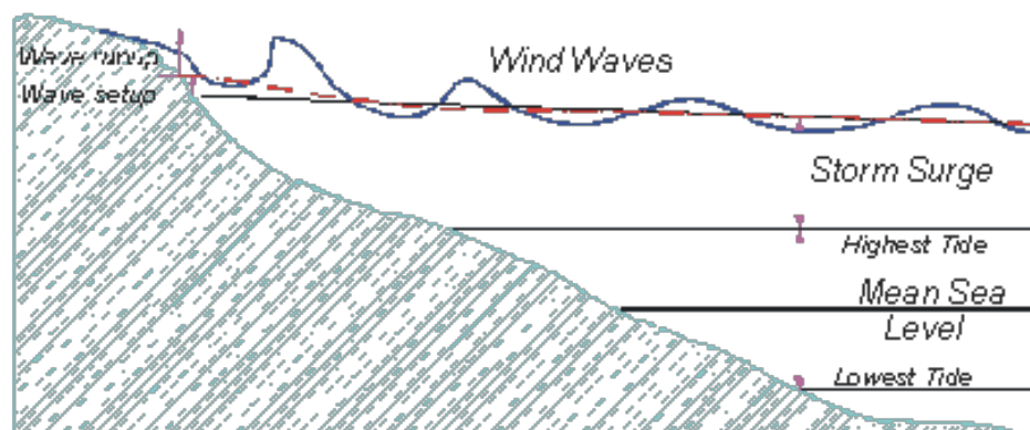
Figure A4.28 Systematic diagram illustrating the contributions to coastal sea level from tides, storm surge and wave processes
