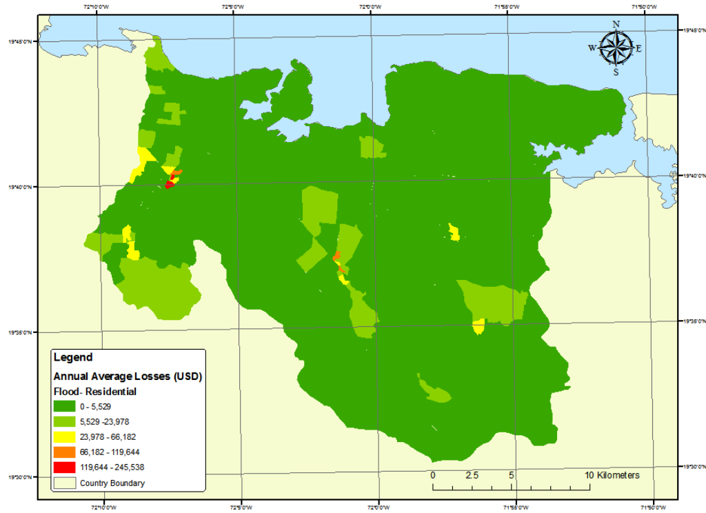
Figure A6.10 Risk Map: AAL for Flooding Hazard, Residential
