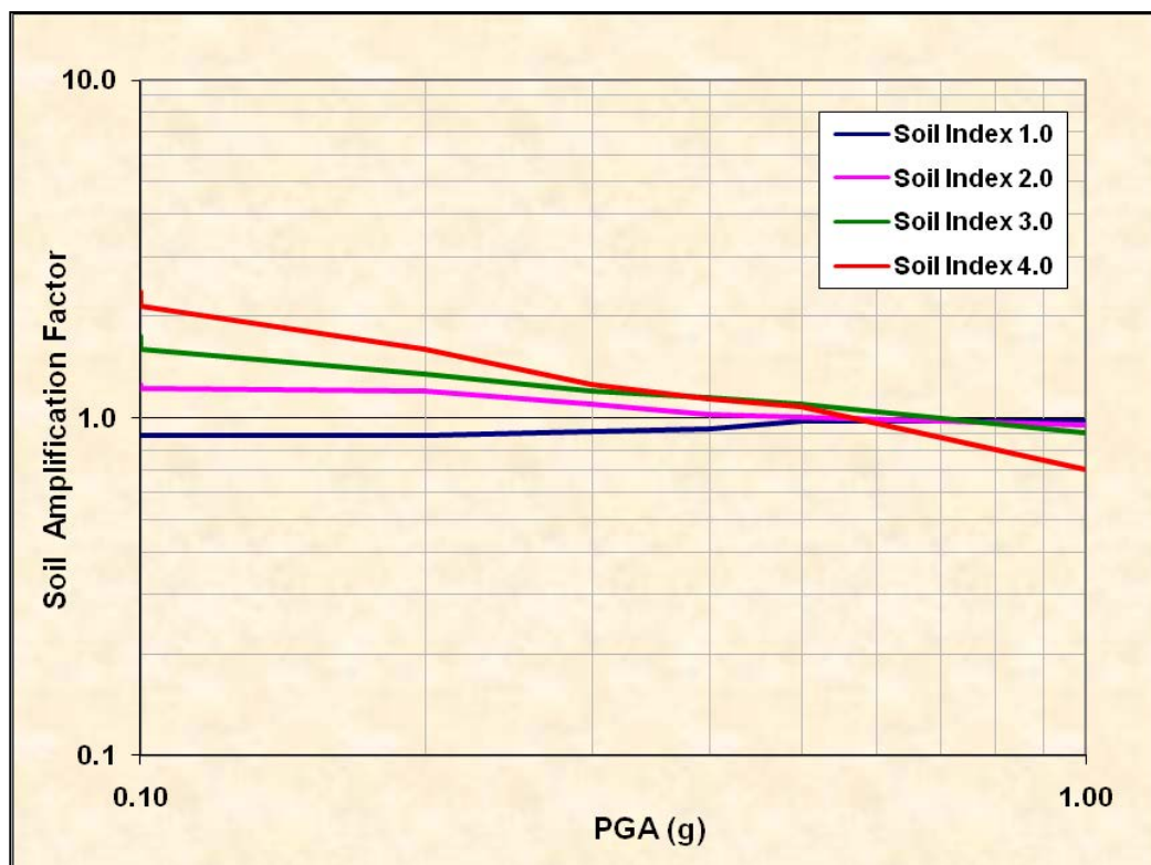
Figure A4.10 Site amplification factors for different soil index values (= VS30 values)
