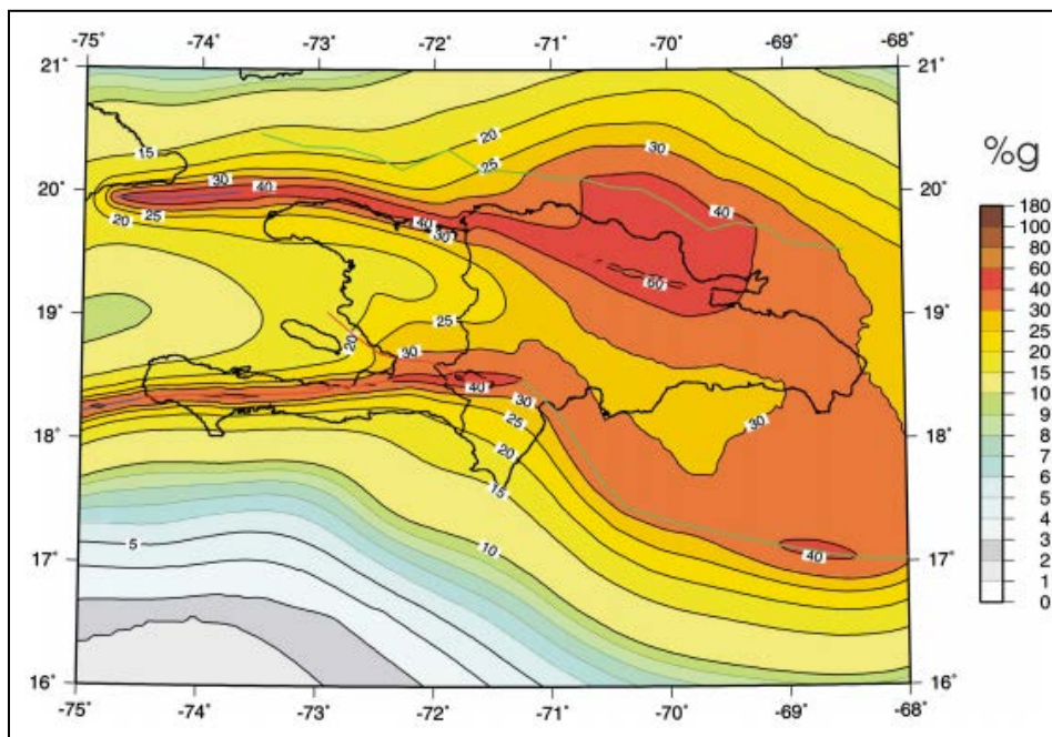
Figure A4.3 PGA (% g) with 10% probability of exceedance in 50 years (475 years return periods)
