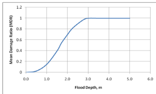
Figure 28 - Example of vulnerability function for Coastal Flood Hazard for low rise masonry structure
