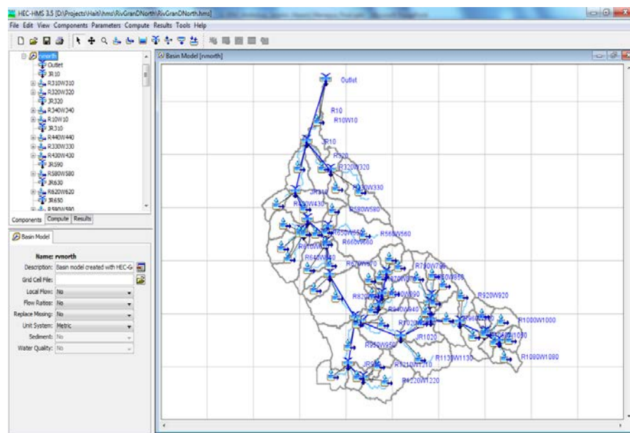
Figure A4.18 HMS set up for River Grand du Nord
