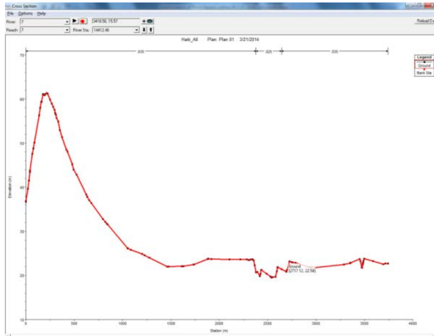
Figure A4.22 Cross section for River Trou du Nord
