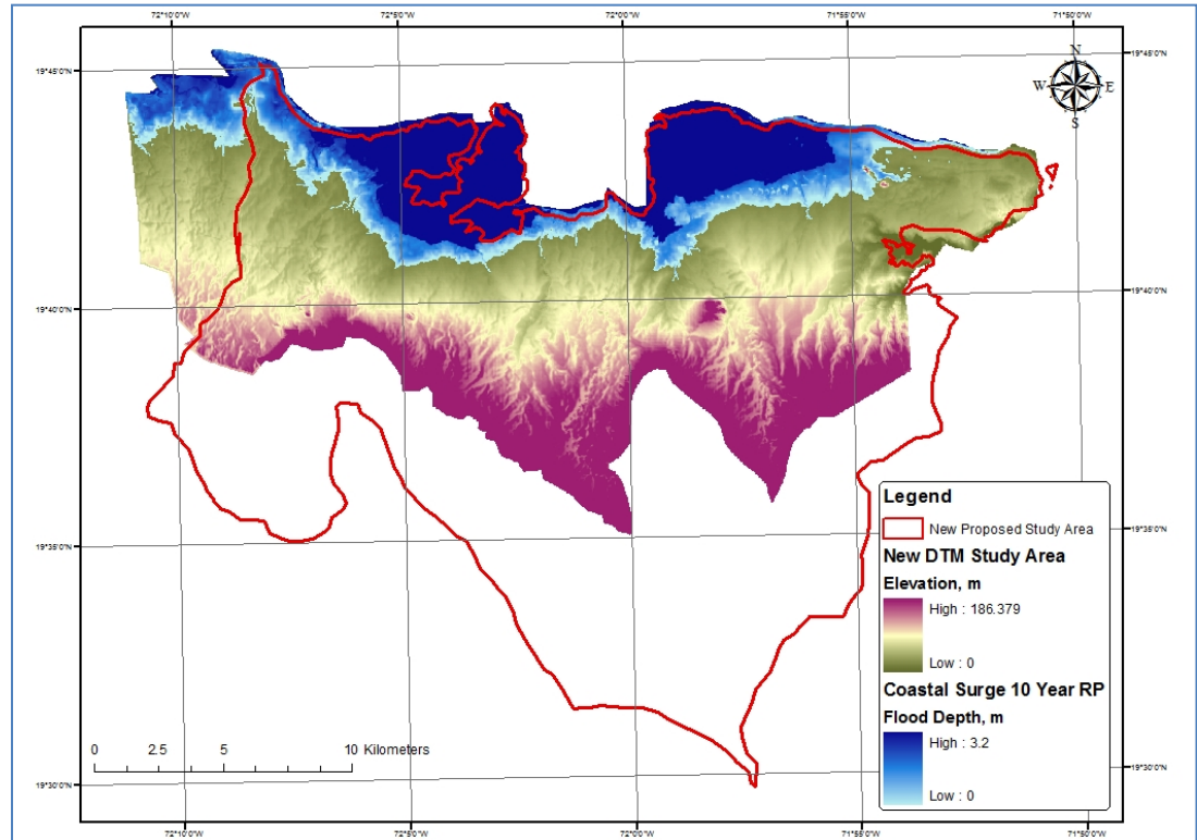
Figure A4.30 10 Year Return Period
