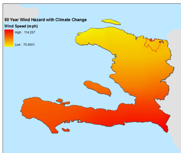
50 Year Wind Hazard Map with climate change
