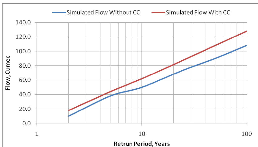
Figure A4.25 Return Period Flows with and without climate change for Trou du Nord river
