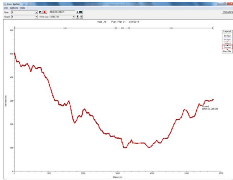
Figure A4.21 Cross section for River Grand du Nord
