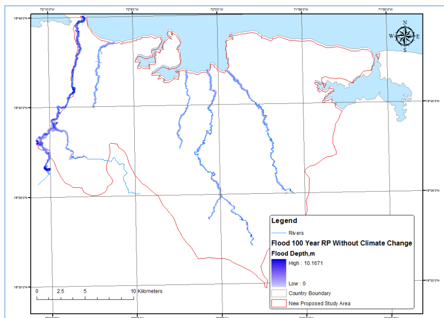
Figure A4.24 Flood Hazard Map without Climate Change 100 year return period
