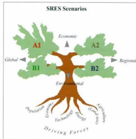
Figure 1.1: Schematic illustration of the four SRES storylines
