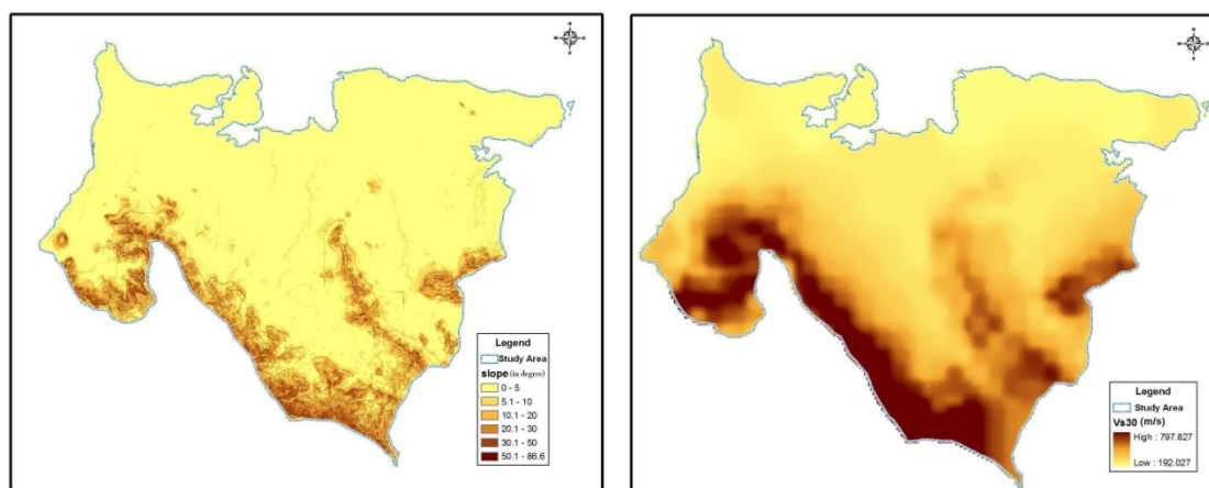
Figure A4.8 The slope map derived from high resolution DEM (left) and distribution of Vs 30 within the study area
