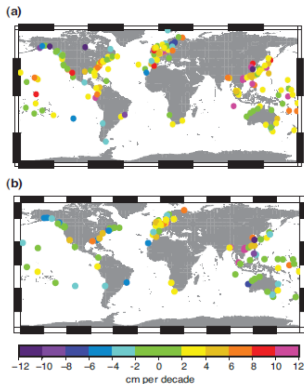
Figure 2.4: Estimated trends (cm per decade) in the height of a 50-year event in extreme sea level from (a) total elevation and (b) total elevation after removal of annual medians. Black dots indicate trends are not significant at the 95% confidence level. Data are from Menéndez and Woodworth (2010).
