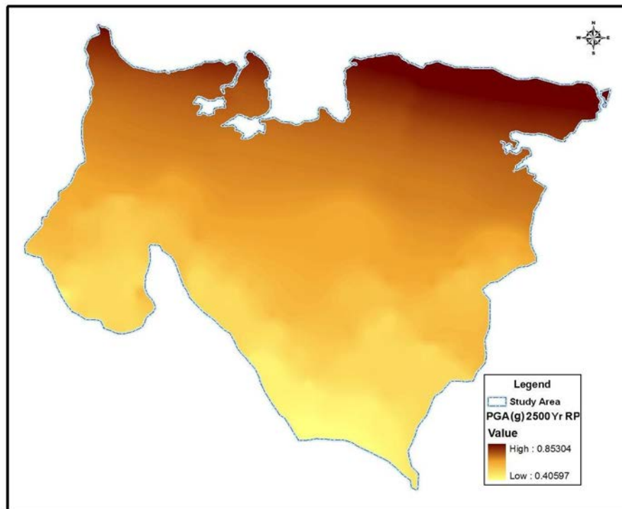
Figure A4.12 PGA probabilistic seismic hazard map for 2% probability in 50 years, i.e. 2,500 year return period
