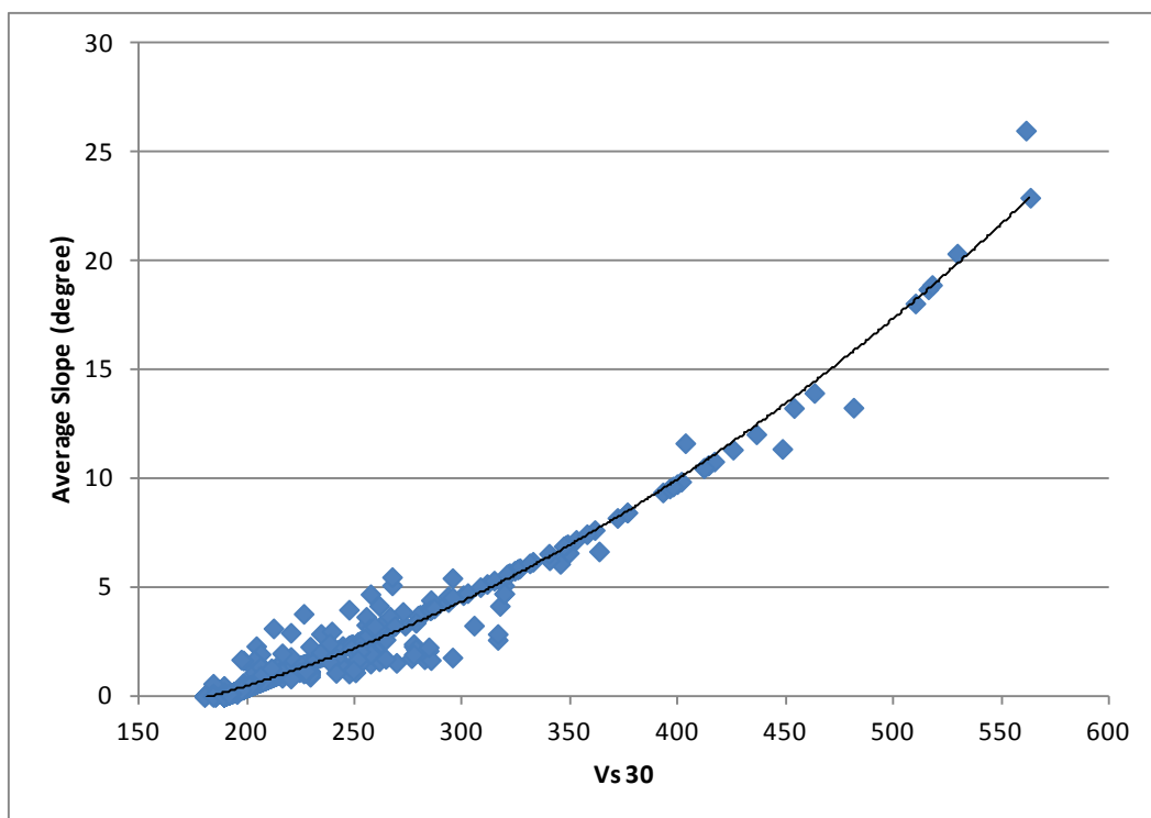
Figure A4.7 Average slope and Vs 30 relationship for the study area
