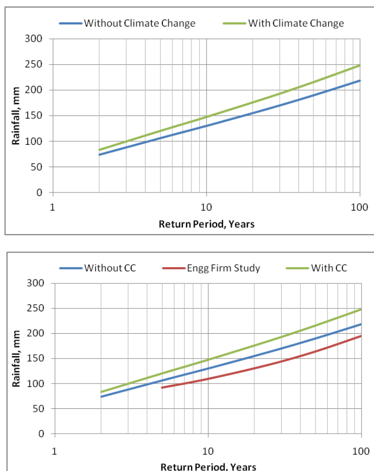
Figure A4.16 Estimated Return Period Rainfalls
