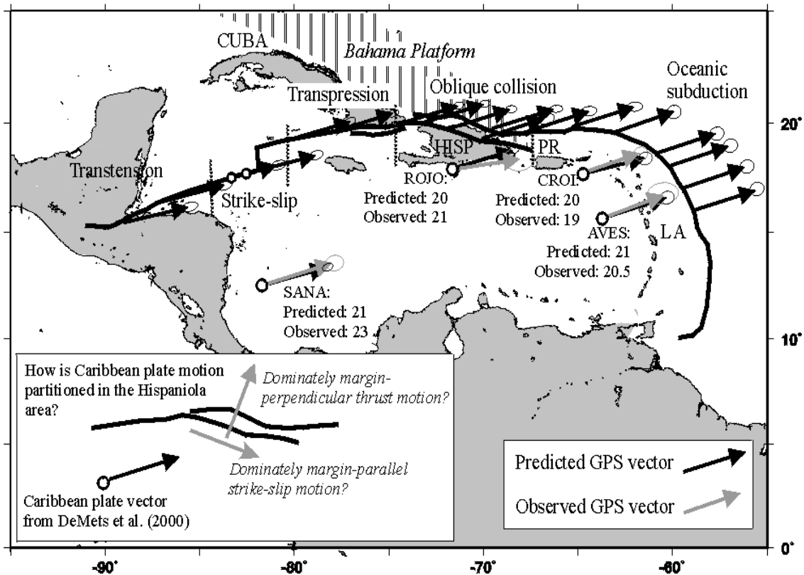
Figure A4.1 Relative vectorial displacement of the Caribbean tectonic plate
