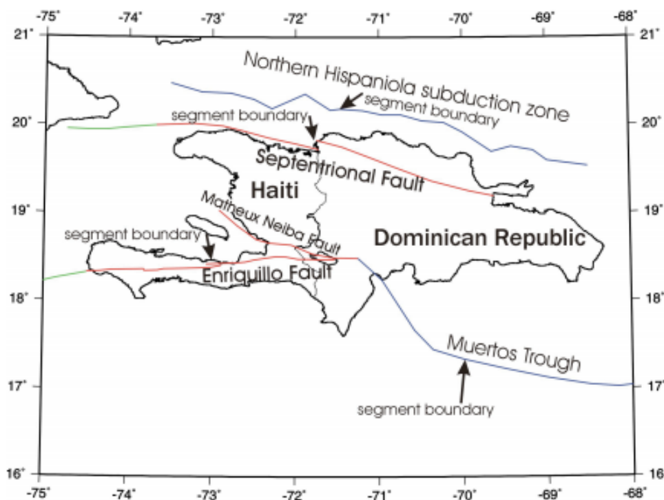
Figure A4.2 Crustal faults and subduction zones used in the hazard maps.
