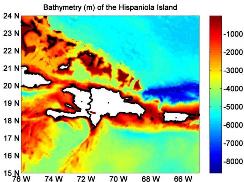
Figure A4.29 Bathymetry of the Island of Hispaniola
