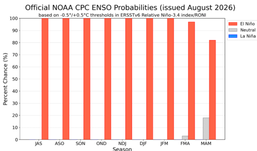
Figure 1. Official ENSO probabilities for the Niño 3.4 relative SST index ( 5^{\circ}\text{N} – 5^{\circ}\text{S} , 170^{\circ}\text{W} – 120^{\circ}\text{W} ) minus tropical mean ( 20^{\circ}\text{N} – 20^{\circ}\text{S} ). Figure updated 13 August 2026. Source: NOAA/CPC
