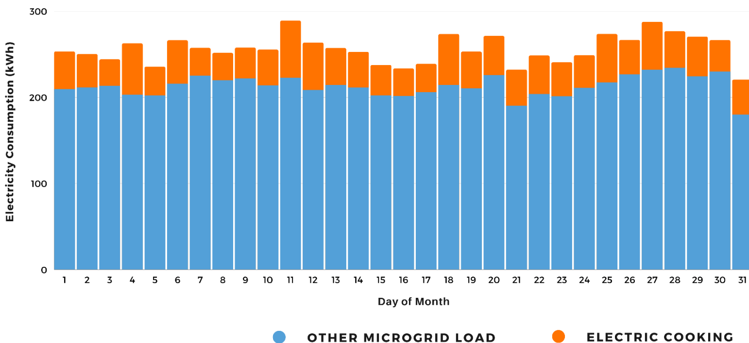
Figure 9: Daily Total Microgrid Electricity Consumption in October
