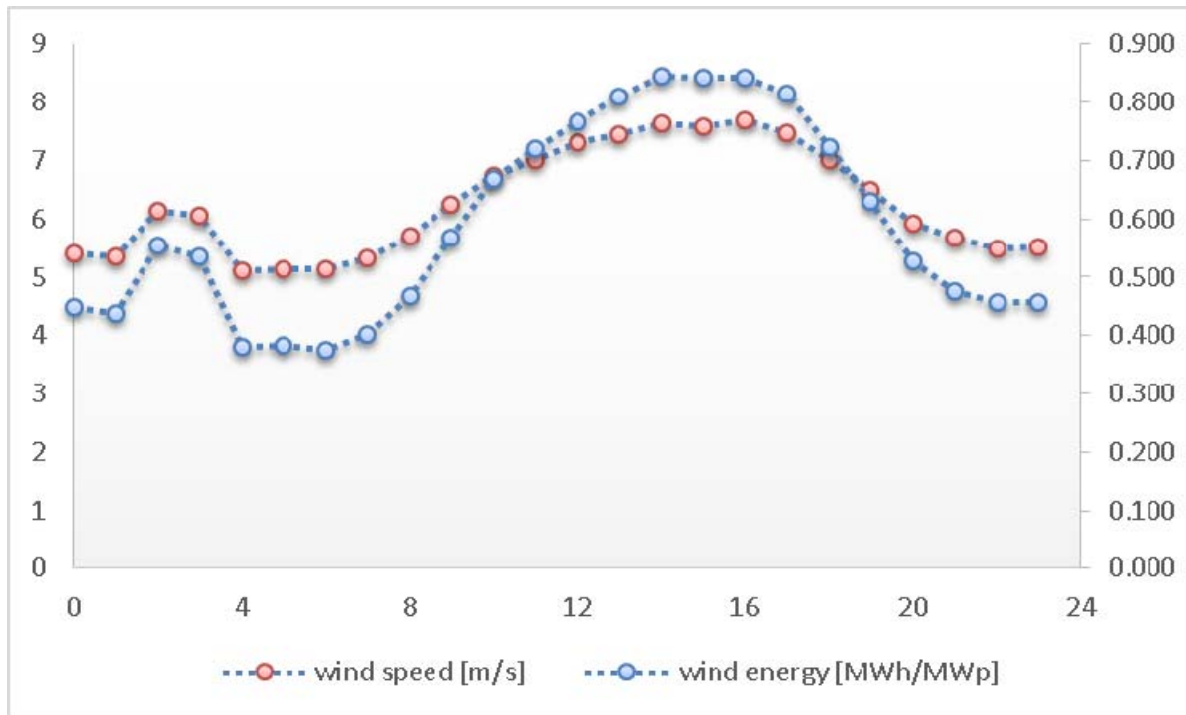
Figure 9. Typical diurnal wind energy profile
